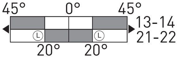
Switching diagram
