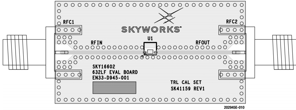
Figure 10. SKY16602-632LF Evaluation Board Assembly Diagram
