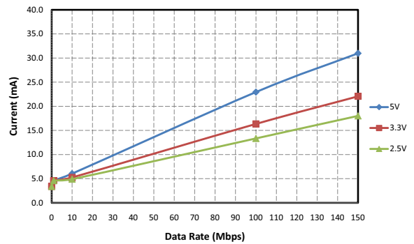
Figure 12. Si8661 Typical V_{DD2} Supply Current vs. Data Rate 5, 3.3, and 2.5 V Operation (15 pF Load)
