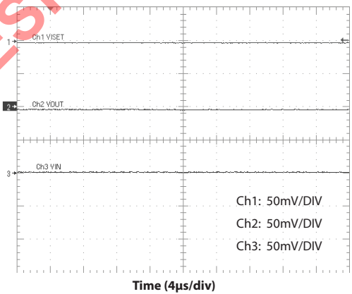
Spotlight 1x Mode Ripple, R_{ISET} = 500m\Omega
