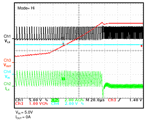
Recovery from OCP ( V_{OUT}=3.3\text{V} )
