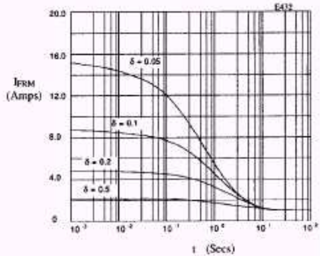
Fig 8. Typical repetitive forward current as a function of pulse width at 100°C; R_{AJL} = 80 \text{ } ^\circ\text{C/W} ; V_{RWM} during 1 - \delta .
