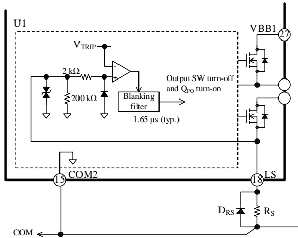
Figure 11-14. Internal Circuit Diagram of LS Pin and Its Peripheral Circuit
