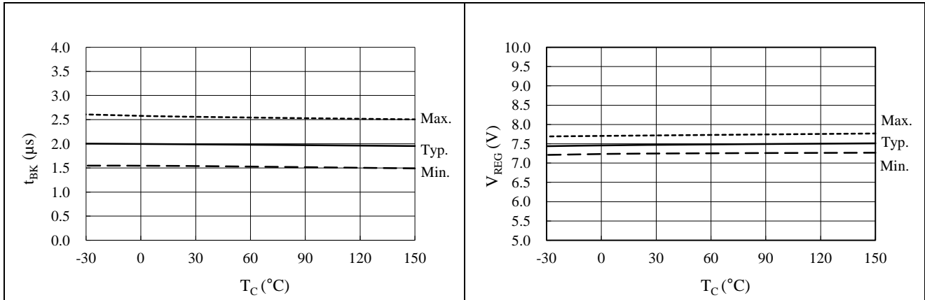
Figure 14-27. OCP Blanking Time, t_{BK(\text{OCP})} vs. T_C ; Current Limit Blanking Time, t_{BK(\text{OCL})} vs. T_C
