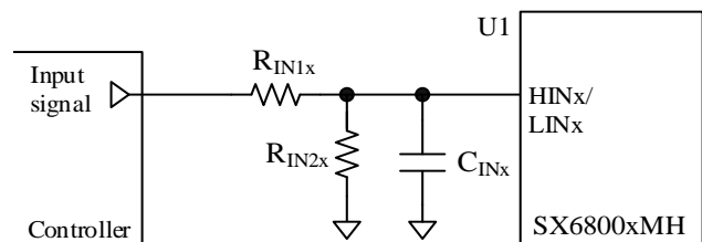
Figure 11-7. Filter Circuit for HIN x or LIN x Pin
