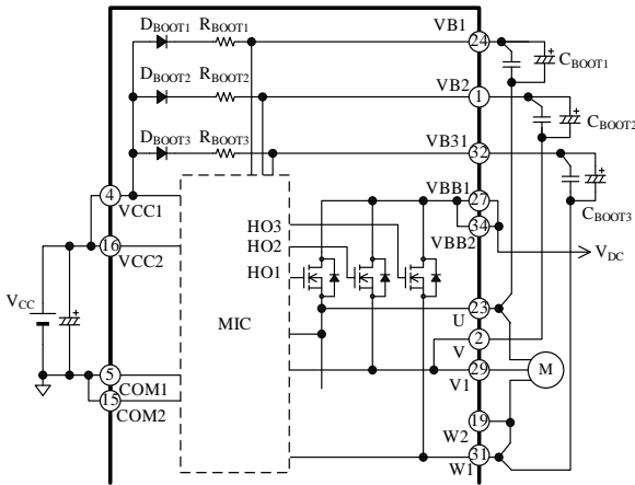
Figure 11-1. Bootstrap Circuit
