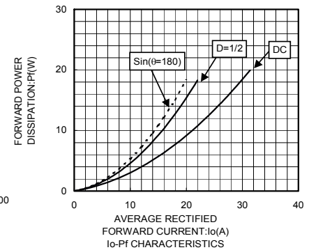
I_o -P CHARACTERISTICS
