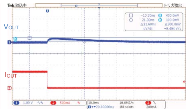
Figure 27. V_{IN} = 230 \text{ Vac} , I_{OUT} = 0.715 \text{ A} \rightarrow 10 \text{ mA}
