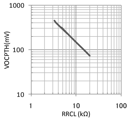
Fig.45 OCP Threshold vs RRCL
