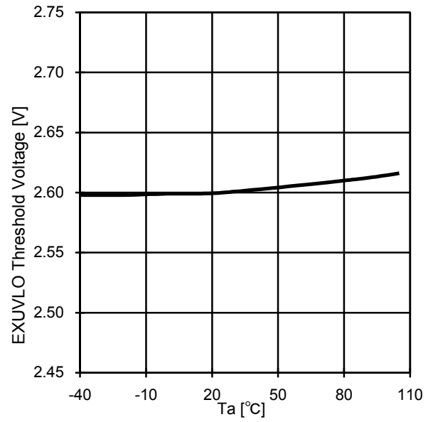
Fig.10 EXUVLO (CTL)-Ta
