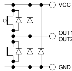
Fig.44 OUT1 / OUT2 (SOP8/HRP7)
