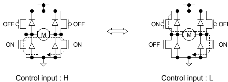
Fig.38 PWM control mode B operation (output stage)
