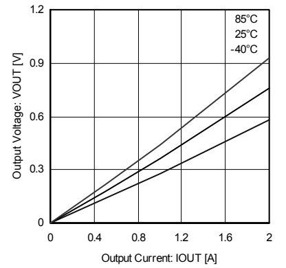
Fig.21 Output low voltage (2A class)
