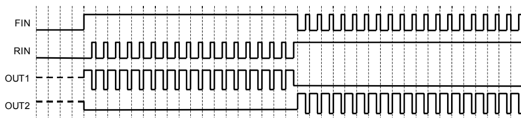
Fig.39 PWM control mode B operation (timing chart)
