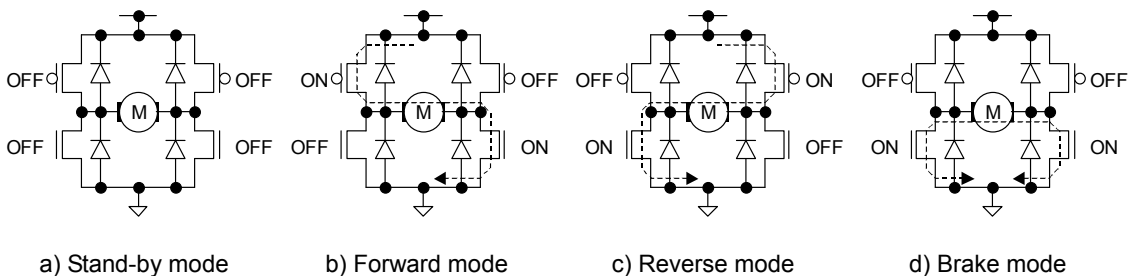
Fig.35 Four basic operations (output stage)
