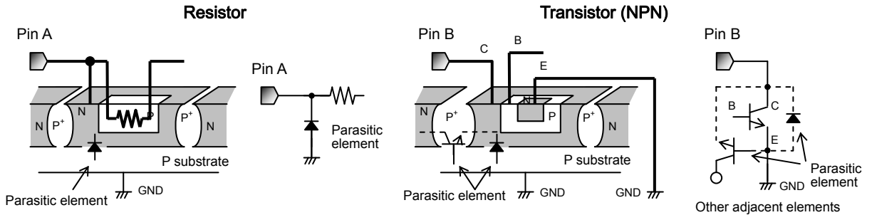
Appendix: Example of monolithic IC structure
