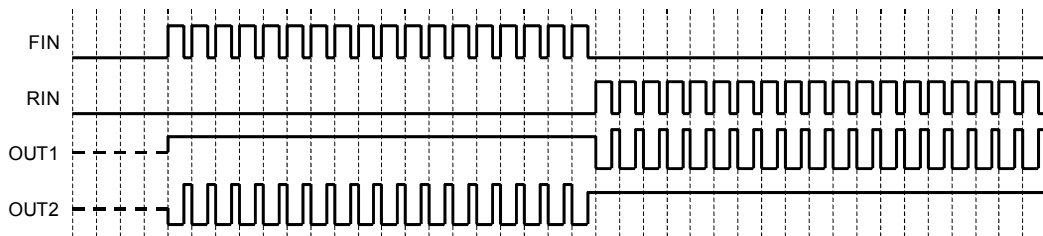
Fig.37 PWM control mode A operation (timing chart)
