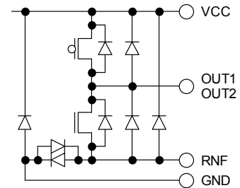
Fig.45 OUT1 / OUT2 (HSOP25/HSOPM28)
