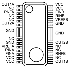
Fig.32 HSOP25
