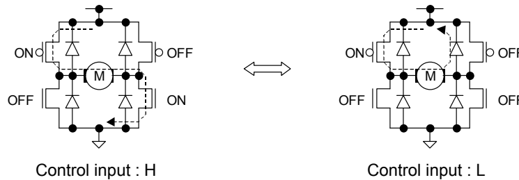
Fig.36 PWM control mode A operation (output stage)
