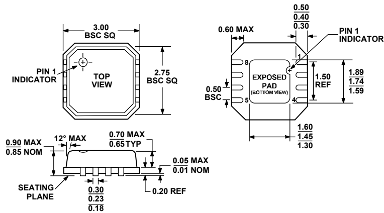
Figure 53. 8-Lead Lead Frame Chip Scale Package [LFCSP_VD] 3 mm x 3 mm Body, Very Thin, Dual Lead (CP-8-2)
