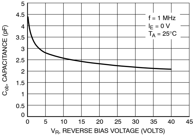
Figure 49. Output Capacitance
