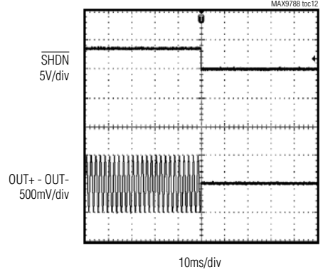
SHUTDOWN WAVEFORM
