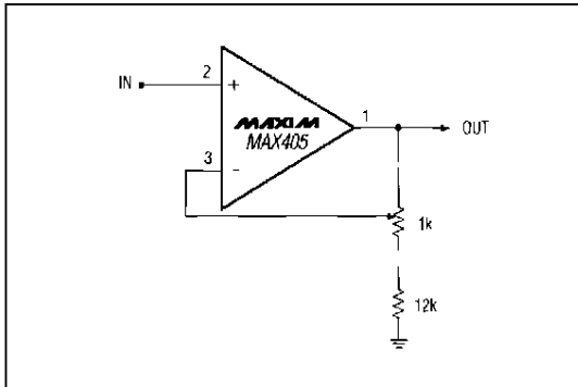
Figure 3. Gain-Trim Circuit
