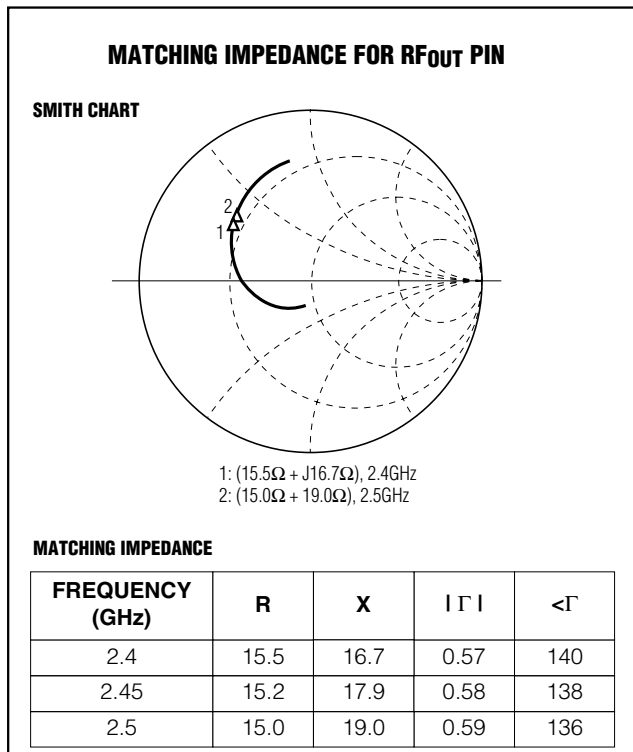
Figure 1. Output Impedance
