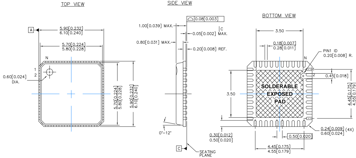
Figure 12. 40-Pin Pb-Free QFN 6 x 6 mm LY40
