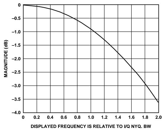
Figure 38. Pass-Band Detail ( R = 63 , HFB 3 Bypassed)
