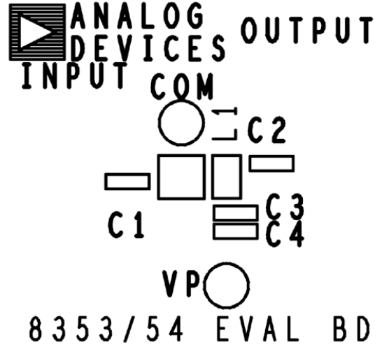
Figure 41. Silkscreen Top
