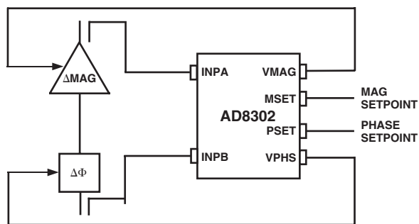
Figure 11. By Applying Overall Feedback to a DUT Via External Gain and Phase Adjusters, the AD8302 Acts as a Controller
