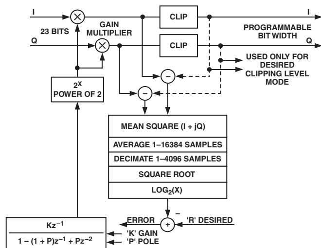
Figure 32. Block Diagram of the AGC
