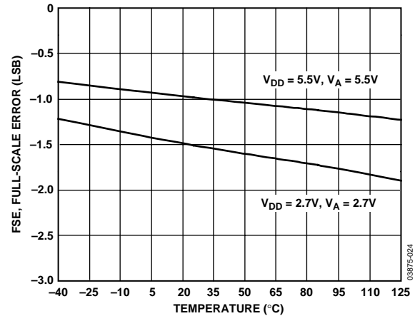
Figure 7. Full-Scale Error vs. Temperature
