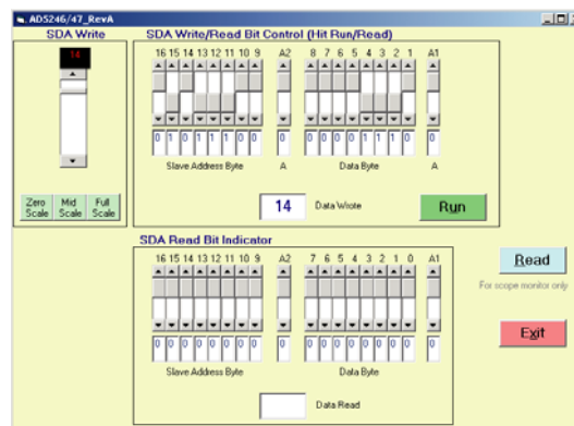
Figure 36. AD5246 Evaluation Board Software
