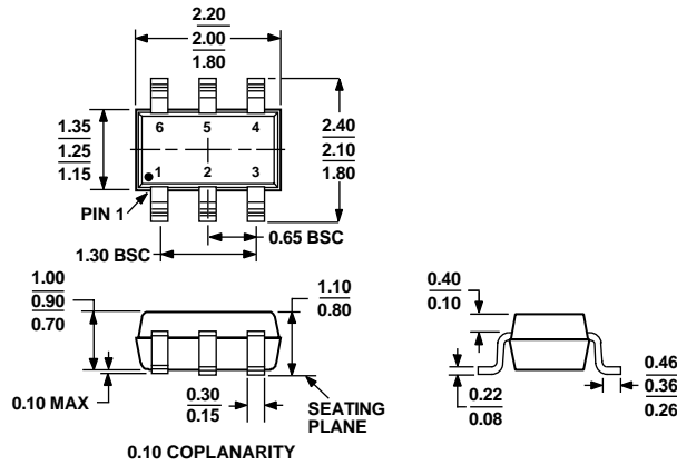
Figure 37. 6-Lead Thin Shrink Small Outline Transistor Package [SC70] (KS-6) Dimensions shown in millimeters
