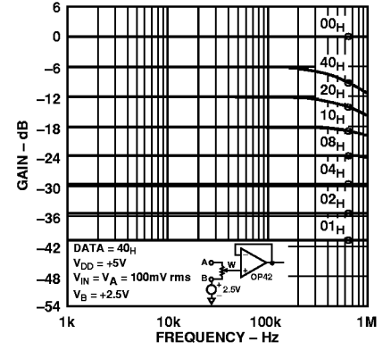
Figure 15. 10 k \Omega Gain vs. Frequency vs. Code
