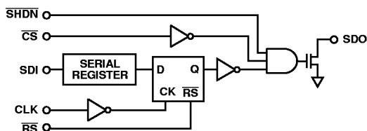
Figure 37. Detail, SDO Output Schematic of the AD5203
