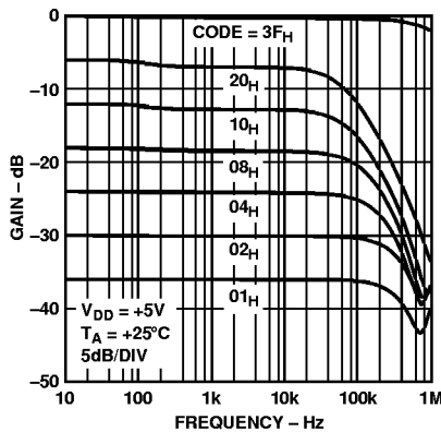
Figure 17. 100kΩ Gain vs. Frequency vs. Code
