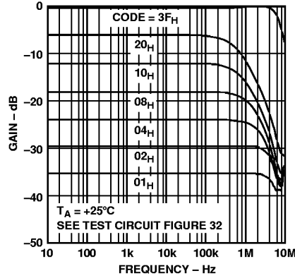
Figure 12. Gain vs. Frequency for R = 10k\Omega
