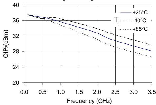
OIP_3 vs. Frequency V_D=4.0\text{ V} , I_D=75\text{ mA}
