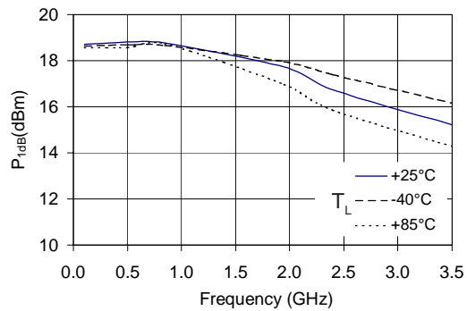
P_{1dB} vs. Frequency V_D=4.0\text{ V} , I_D=75\text{ mA}
