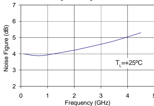
Noise Figure vs. Frequency V_D=4.0\text{ V} , I_D=75\text{ mA}
