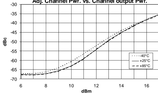
IS-95 @ 850MHz Adj. Channel Pwr. vs. Channel output Pwr.
