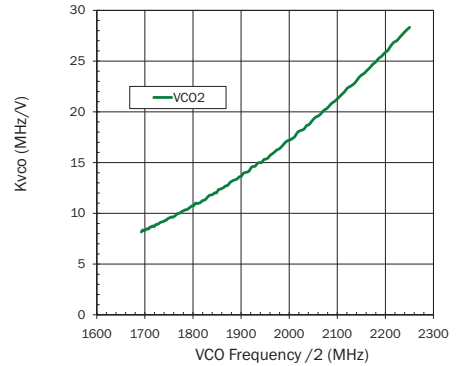
VCO2 Frequency versus Kvco LO Divide by 2
