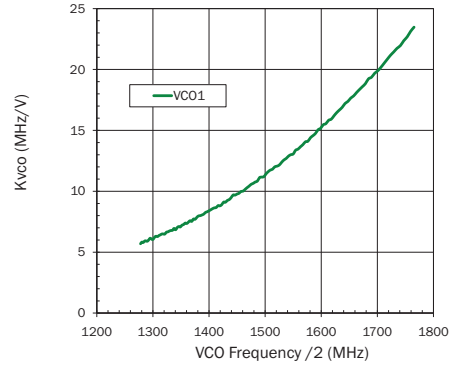
VCO1 Frequency versus Kvco LO Divide by 2
