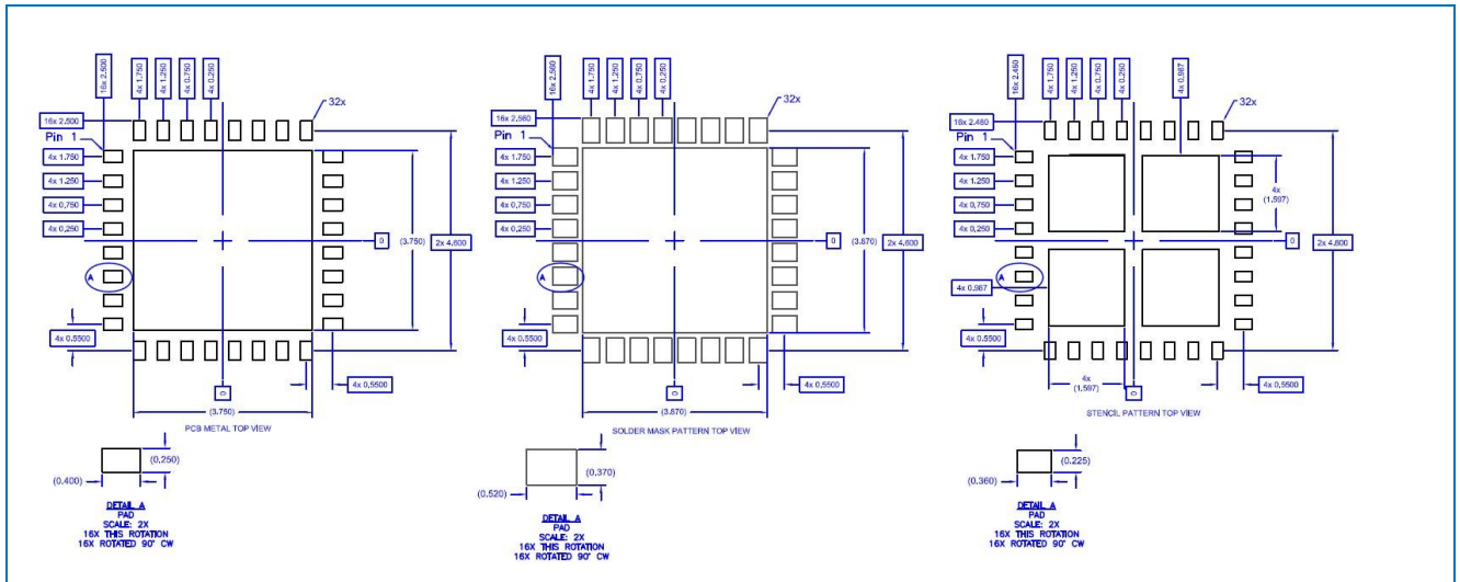
Figure 2. Stencil Recommendation
