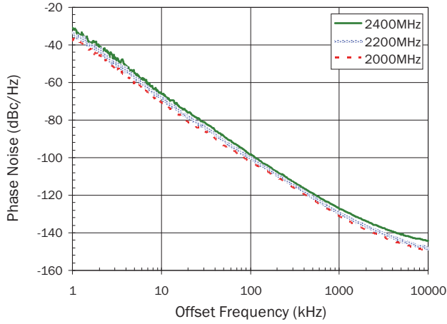
VCO2 Open Loop Phase Noise
