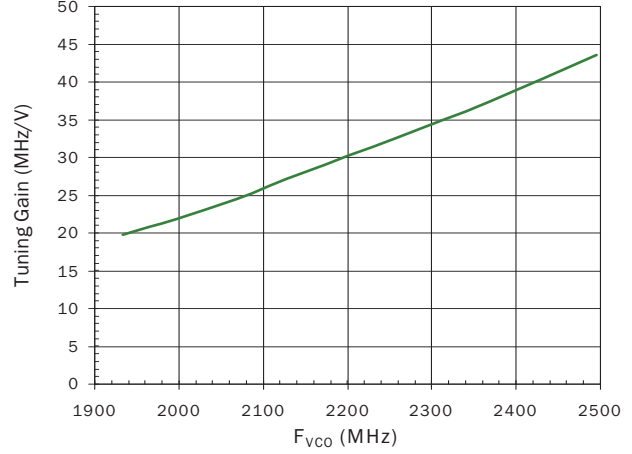
VCO2 Tuning Gain versus Frequency
