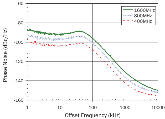
VC03 With Active Loop Filter
