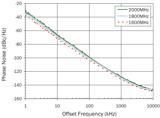
VCO3 Open Loop Phase Noise
