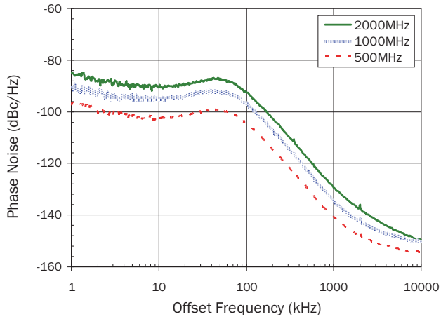
VC02 With Active Loop Filter
