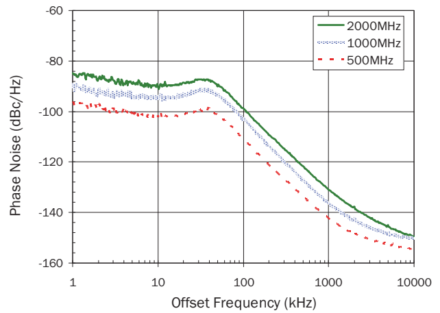
VC02 With Passive Loop Filter
