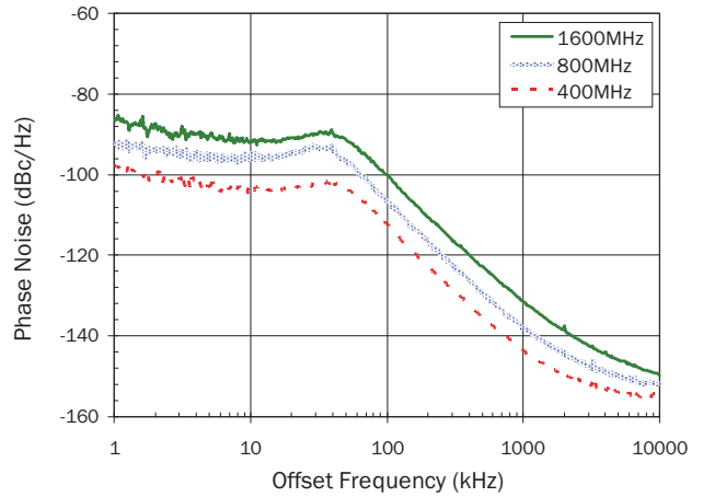
VC03 With Passive Loop Filter
