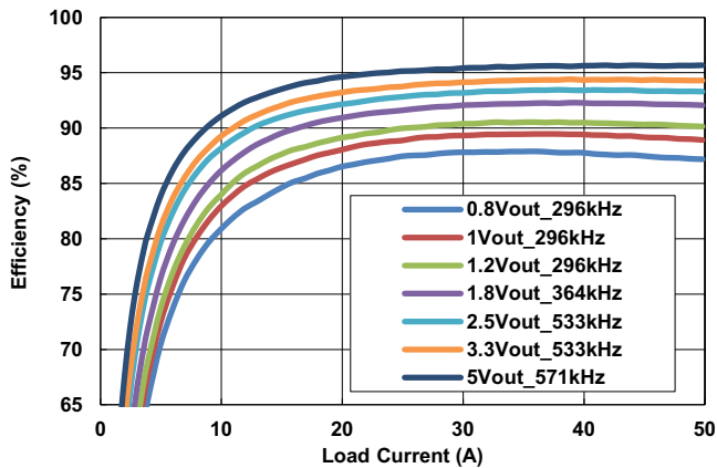
Figure 20. Efficiency vs Output Current at V_{IN} = 12V for Various Output Voltages
