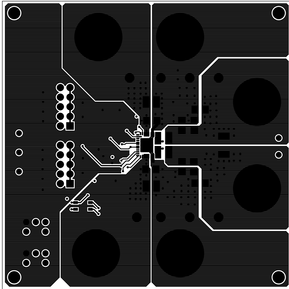
FIGURE 3. TOP LAYER
