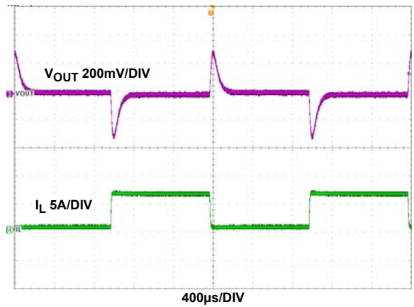
FIGURE 22. LOAD TRANSIENT, I_O = 0A TO 6A, 1A/µs, CCM
