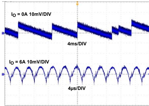
FIGURE 17. OUTPUT RIPPLE, MODE = DEM
