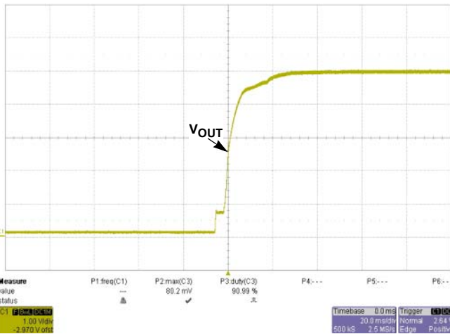
FIGURE 7. START-UP (30ms) AT V_{IN} = 36V @ I_O = 0A
