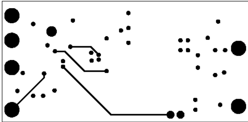
FIGURE 10. ISL6406EVAL1 - LAYER 4
