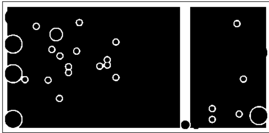
FIGURE 9. ISL6406EVAL1 - LAYER 3
