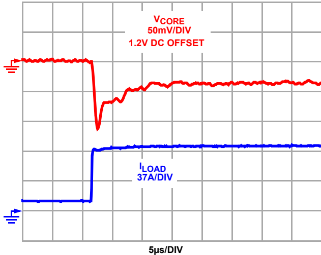
FIGURE 12. CORE LOAD TRANSIENT: 10A DC AND 70A LOAD APPLY (400A/ \mu s)
