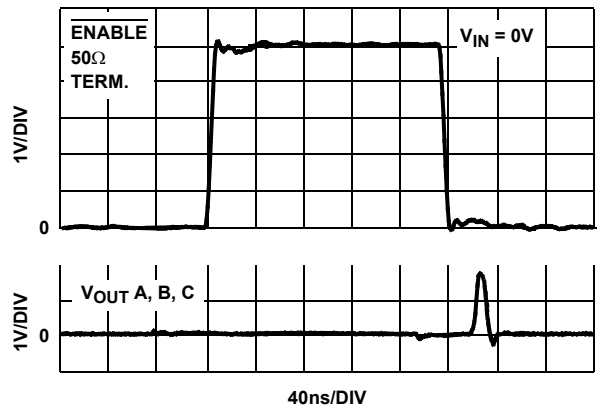
FIGURE 33. MUX 2: ENABLE SWITCHING GLITCH V_{IN} = 0V
