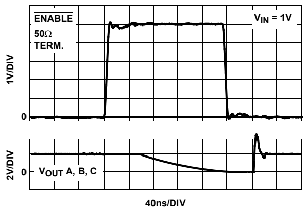
FIGURE 35. MUX 2: ENABLE TRANSIENT RESPONSE V_{IN} = 1V
