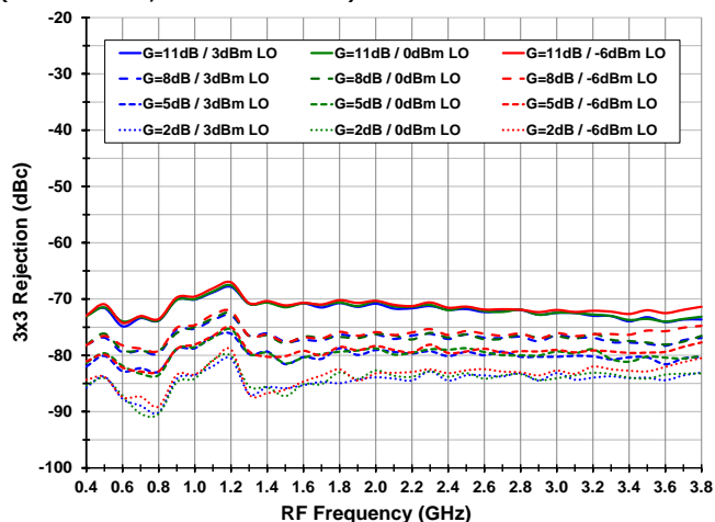
3x3 Rejection vs. LO Power and Gain Setting (Vcc = 3.15, Tcase = 105C)
