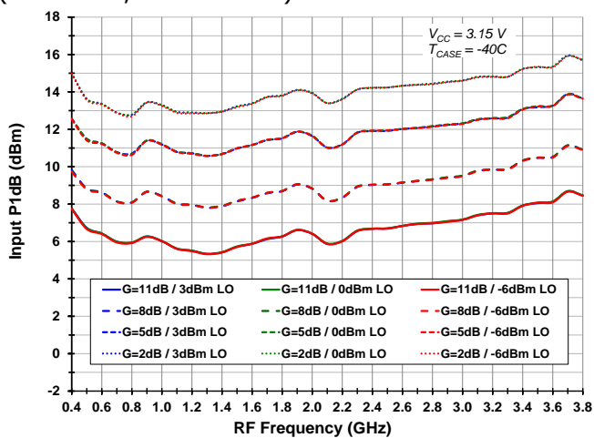
Input P1dB vs. LO Level and Gain Setting (Vcc = 3.15, Tcase = -40C)
