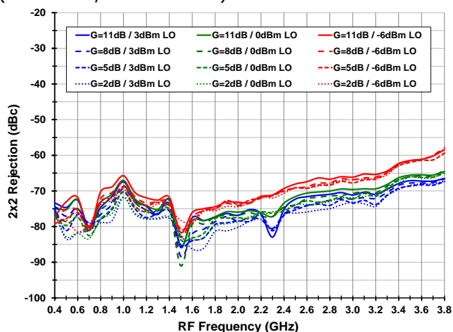
2x2 Rejection vs. LO Power and Gain Setting (Vcc = 3.15, Tcase = 105C)
