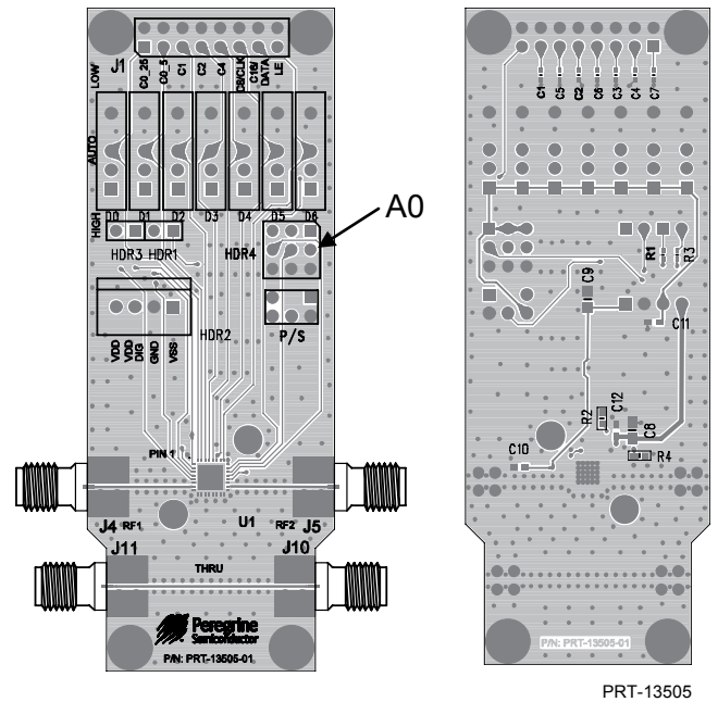
Figure 30. Evaluation Board Layout
