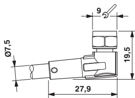
Dimensional drawing
