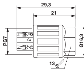
Dimensioned drawing
