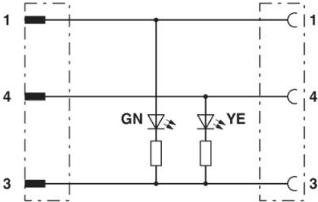
Contact assignment of M12 plugs / M8 sockets
