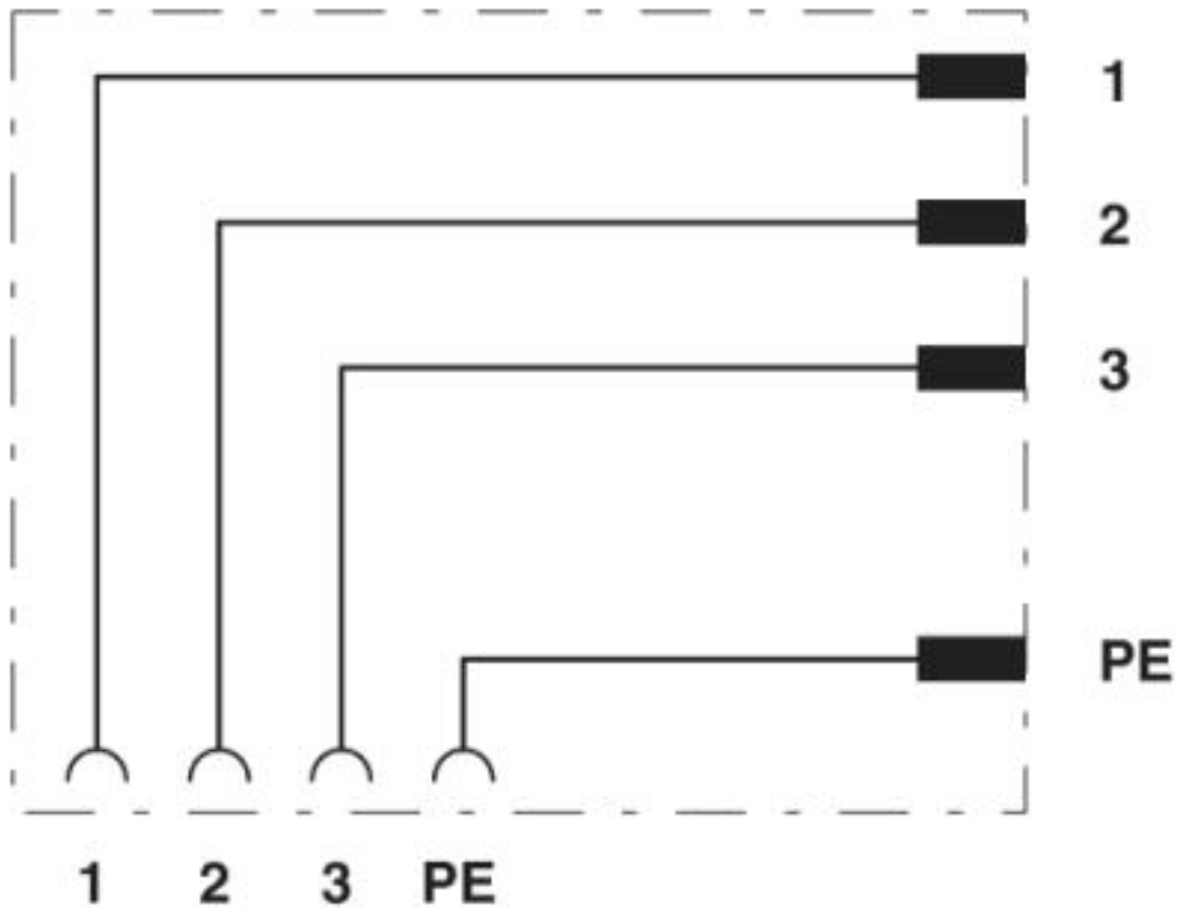
Circuit diagram
