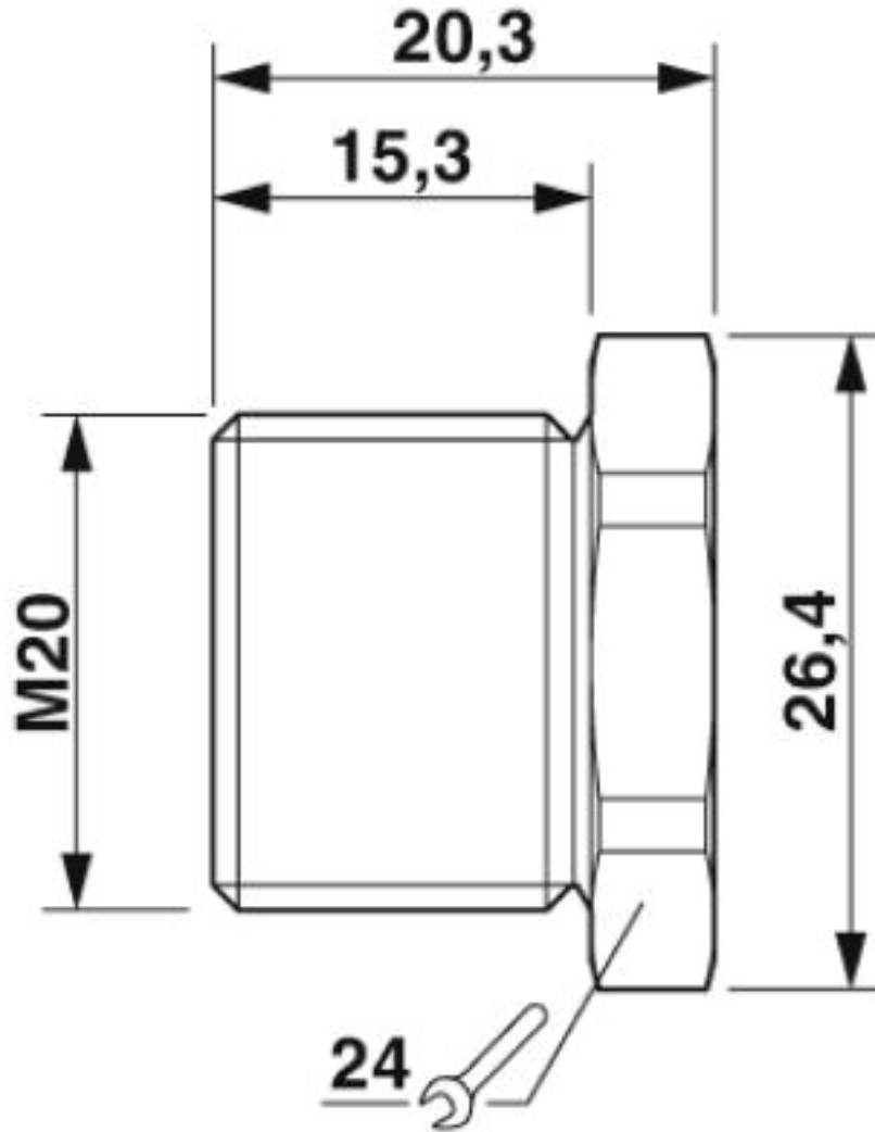
Dimensional drawing
