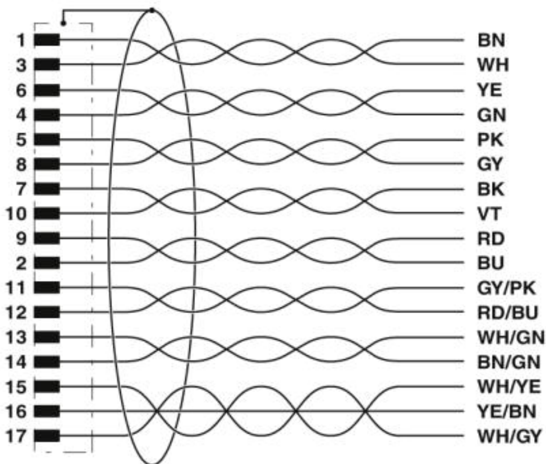
Circuit diagram
