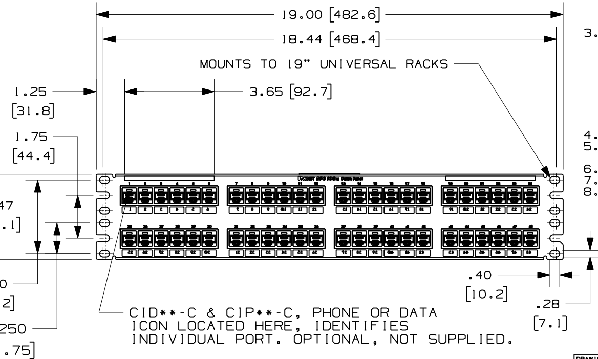
FIGURE 1 DP5e 48 PORT PATCH PANEL
