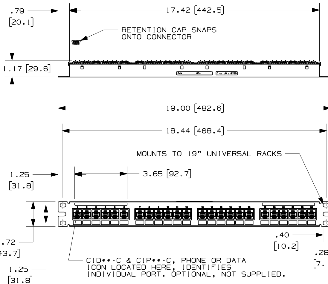
FIGURE 1 DP5e 24 PORT PATCH PANEL
