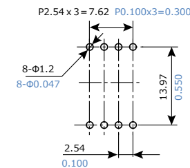
Recommended PC board pattern (BOTTOM)
