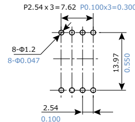
Recommended PC board pattern (BOTTOM)
