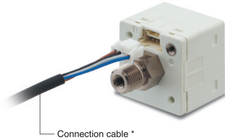
Connection cable *
