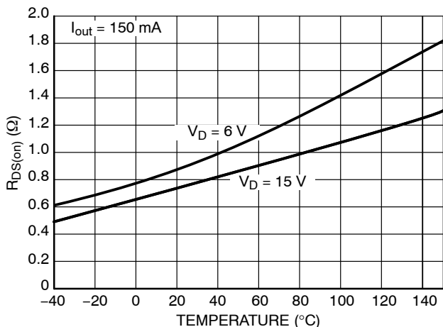
Figure 3. R_{DS(on)} vs. Temperature
