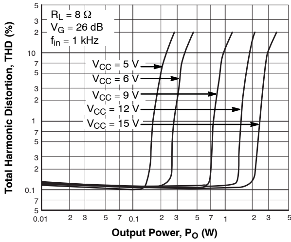
Figure 16. THD - P O
