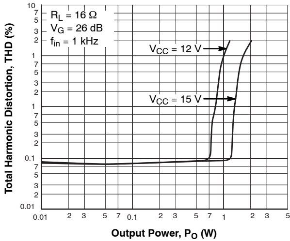
Figure 18. THD - P O
