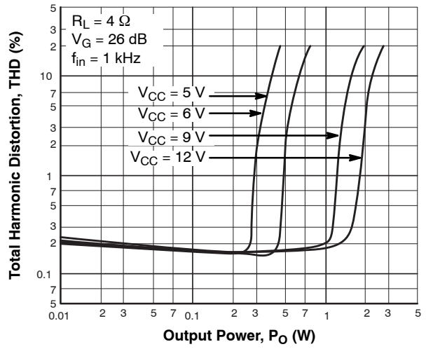
Figure 17. THD - P O
